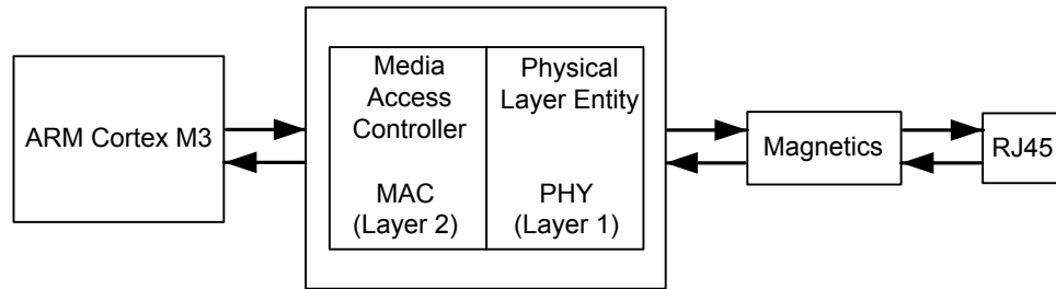
Figure 14-1. Ethernet Controller
